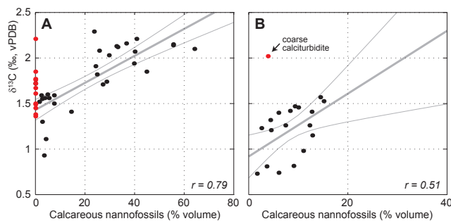
Fig. 8. Carbon isotope composition ( \delta^{13}\text{C} ) of lime mudstone plotted against the abundance of calcareous nannofossils at Pizzo Mondello ( A ) and Pignola-Abriola ( B ). The \delta^{13}\text{C} is clearly correlated with nannofossil abundance (see correlation coefficients ( r )) which are both significantly different from zero at the 95 % level. Linear fit is plotted with 90 % error bounds. Twelve samples of Pizzo Mondello without nannofossils and one sample of Pignola from a 2 m thick coarse calciturbidite are marked in red and were excluded from computation.
