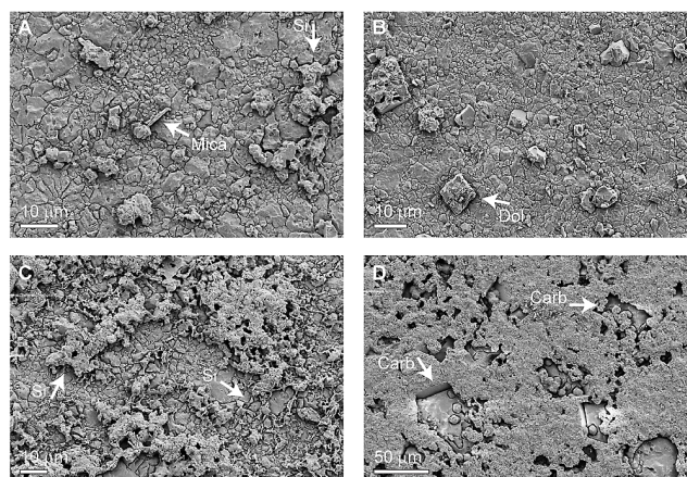
Fig. 4. Examples of diagenetic alteration of micrite and microsparite. (A) Slightly silicified sample with minor terrigenous component (mica crystal in the center of the frame). Calcareous nannofossils are easily visible. Silicified patches (Si) stick out of the sample plain because of etching. Pignola-Abriola section, Parvigondolella andrusovi – Misikella hernsteini conodont zone, late Norian, 33.3 m in Fig. 3. (B) Dolomite rhombohedrons (Dol) in microsparitic lime mudstone. Pignola-Abriola section, Misikella ultima conodont zone, Rhaetian, 58.8 m in Fig. 3. (C) Silicified lime mudstone. Silica (Si) occupies a large part of the rock volume in this frame, and can be found in interstitial position between carbonate crystals or as patches. Pignola-Abriola section, Parvigondolella andrusovi – Misikella hernsteini conodont zone, late Norian, 40.7 m in Fig. 3. (D) Strongly silicified sample. Carbonate (Carb) is only present as a few crystals that partially engulf silica with spheroidal shape (chalcedony?). Locally, carbonate crystal faces are instead preserved. Pignola-Abriola section, Parvigondolella andrusovi – Misikella hernsteini conodont zone, late Norian, 45.1 m in Fig. 3.
