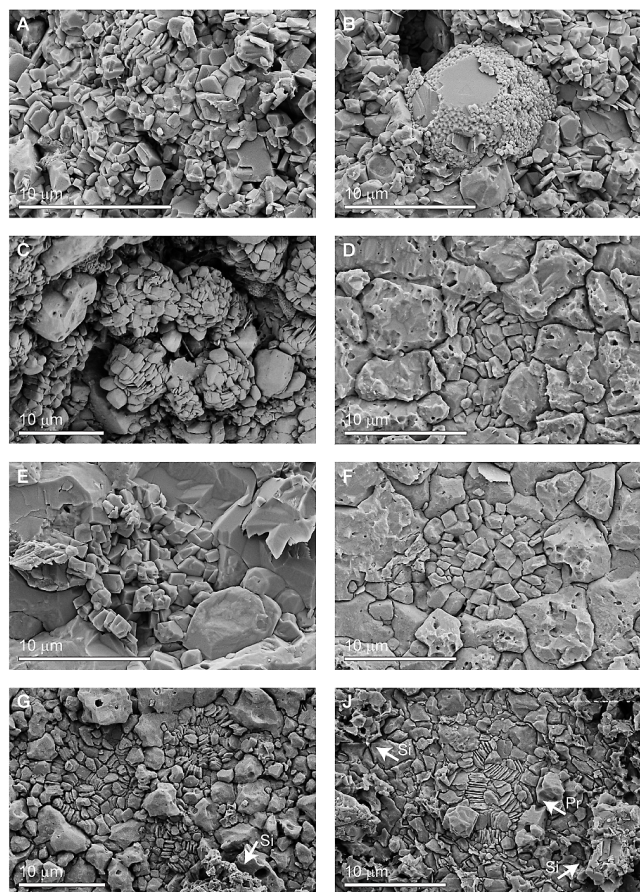
Fig. 6. Calcareous nannofossils from the late Norian and Rhaetian of the southern Apennines and Sicily. (A) Scales of Prinsiosphaera from the Misikella ultima conodont zone, Rhaetian of Pizzo Mondello, 54.5 m in Fig. 2: fresh broken sample. In this example, Prinsiosphaera “calcispheres” cannot be discerned either because they were disarticulated, or because they have been compacted during burial. (B) Thoracosphaera geometrica from the Misikella ultima conodont zone, Rhaetian of Pizzo Mondello, 54.5 m in Fig. 2: fresh broken sample. This and other nannofossils, different from Prinsiosphaera , are minor constituents of the carbonate sediment at Pizzo Mondello and were not recognized at Pignola-Abriola. (C) Prinsiosphaera from the Misikella posthernsteini conodont zone, Rhaetian of Pizzo Mondello, 40.25 m in Fig. 2: surface of “calcispheres” within a primary cavity of the sediment. (D) Prinsiosphaera from the Parvigondolella andrusovi – Misikella hernsteini conodont zone, late Norian of Pizzo Mondello, 19.95 m in Fig. 2: polished and etched sample. (E, F) Prinsiosphaera from the Mockina bidentata conodont zone, late Norian of Pizzo Mondello, 13.1 m in Fig. 2: comparison of the freshly broken sample (E) and polished and etched sample (F) . (G) Three specimens of Prinsiosphaera with different diameters from the Mockina bidentata conodont zone, late Norian of Pignola-Abriola, 23.7 m in Fig. 3. This sample was polished and etched. Silicification (Si) is visible. (J) Prinsiosphaera (Pr) and silicified patches (Si) from the Misikella posthernsteini conodont zone, Rhaetian of Pignola-Abriola, 52.1 m in Fig. 3. Polished and etched sample.
