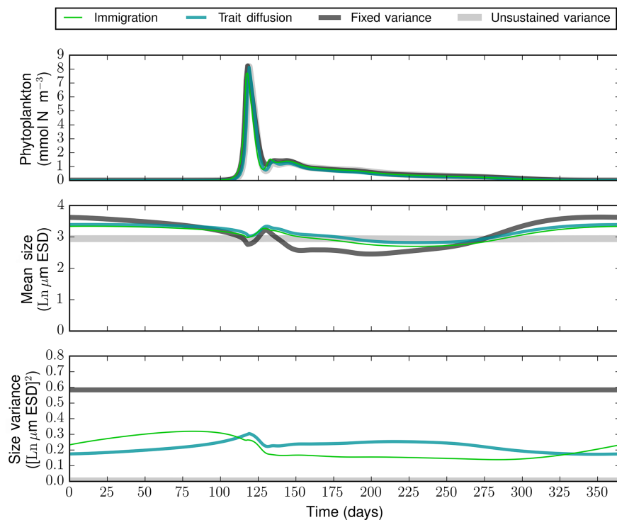
Figure 6. Dynamics of the size-structured phytoplankton community and its functional size diversity for the four variance treatments (see Sect. 2.1.3), named unsustained and fixed variance, trait diffusion, and immigration.
