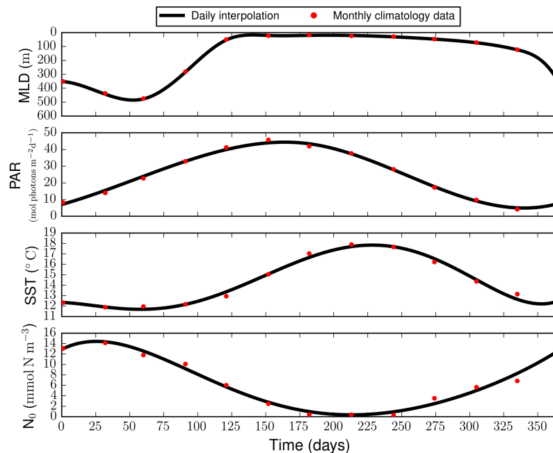
Figure 2. Temporal variation of the environmental variables. The monthly climatology data (red dots) are spatially averaged over the test location (square boxes in Fig. 1). The interpolation (continuous line) is obtained with a third- (MLD and PAR) and a fifth-order (SST and N_0 ) polynomial.
