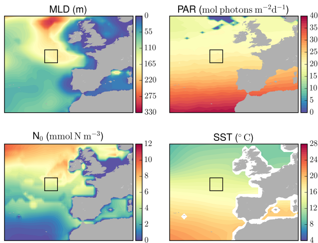
Figure 1. Environmental forcing variables considered in PhytoSFDM. The data shown are the annual average of mixed-layer depth (MLD), photosynthetic active radiation (PAR), sea surface temperature (SST), and nitrogen concentration below the mixed layer ( N_0 ). The square boxes mark the location of the test-case simulation.
