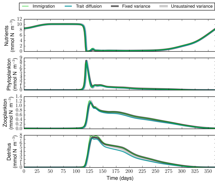
Figure 5. Nutrient, phytoplankton, zooplankton, and detritus dynamics over a seasonal cycle for the four variants of the aggregate model (see Sect. 2.1.3), named unsustained and fixed variance, trait diffusion, and immigration.
