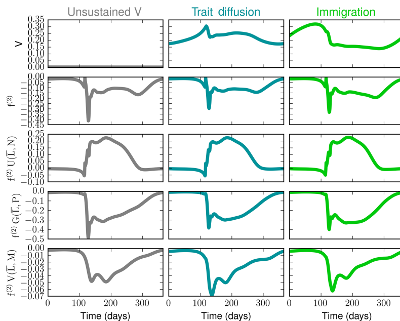
Figure 8. Components of the size variance ( V ), where f^{(2)} is the second derivative of the fitness function with respect to the trait; f^{(2)}U(\bar{L}, N) , f^{(2)}G(\bar{L}, P) , and f^{(2)}V(\bar{L}, M) are, respectively, nitrogen uptake, zooplankton grazing, and phytoplankton sinking components of f^{(2)} .
