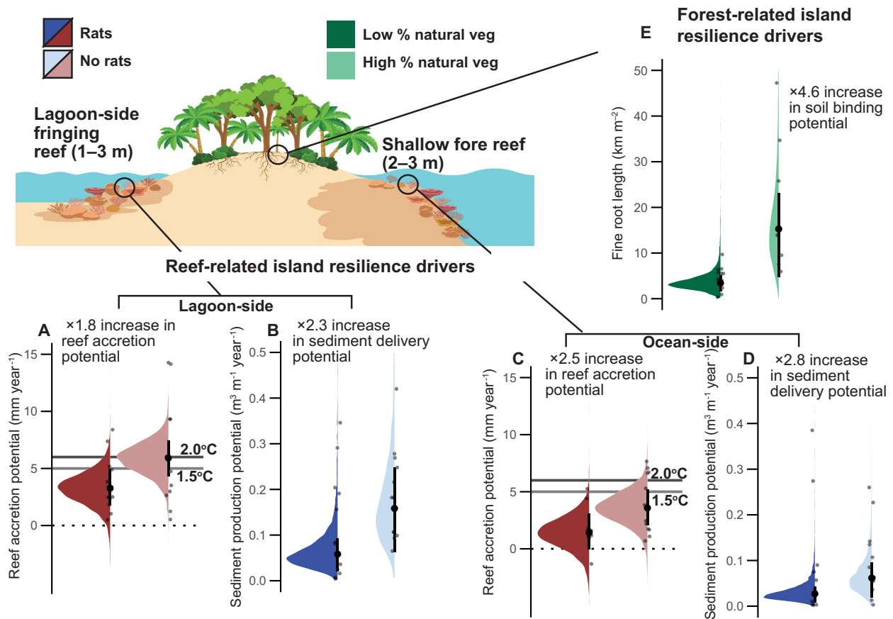
Fig. 4. Geo-ecological functions enhanced by seabirds and native vegetation. Reef accretion potential (RAPmax) on (A) lagoonal and (C) forereef sites adjacent to islands with and without invasive rats ( n = 48 transects across six islands in the Chagos Archipelago). Horizontal gray lines denote projected rate of sea-level rise (mm year -1 ) for the central Indian Ocean in 2100 under 1.5° and 2.0°C warming scenarios. Values of constituent components of reef accretion potential per site are available in table S2. Sediment production potential on (B) lagoonal and (D) forereef sites adjacent to islands with and without invasive rats ( n = 47 transects across six islands in the Chagos Archipelago). (E) Fine root length measured in forest plots ( n = 19 across five islands in Teti'aroa) above and below a 75% native vegetation cover threshold (split also by rat status in table S3). Half-eye plots depict the Bayesian posterior distributions, the median (large point), 75% credible intervals (lines around the medians), and raw data points (small points). All data are analyzed using Bayesian hierarchical models.
