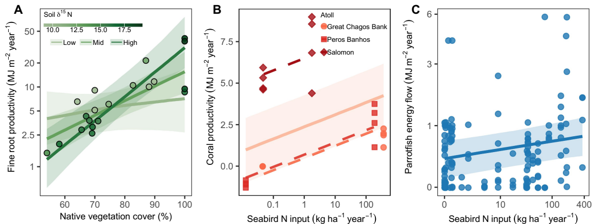
Fig. 2. Primary productivity and animal energy flow on islands and surrounding coral reefs in relation to seabird nutrient inputs and native vegetation cover. (A) Relationship between native vegetation cover and fine root productivity across three representative soil \delta^{15}\text{N} values indicative of differing seabird nutrient inputs (low = mean - 1 SD, mid = mean, high = mean + 1 SD) with 75% Bayesian credible intervals ( n = 20 plots across five islands in Teti'aroa, colored by gradient in soil \delta^{15}\text{N} ). (B) Relationship between seabird nitrogen input to islands and coral community primary productivity on adjacent coral reefs, with 75% Bayesian credible intervals. Solid line = global trend, dotted lines = atoll-level trends due to differing intercepts ( n = 24 transects across six islands in the Chagos Archipelago). (C) Relationship between seabird nitrogen input to islands and parrotfish energy, with 75% Bayesian credible intervals ( n = 134 transects across 27 islands in all three study locations). All data are analyzed using Bayesian hierarchical models.
