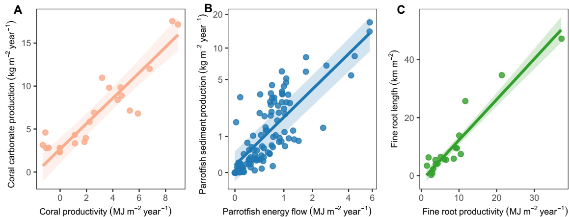
Fig. 3. Scaling of primary productivity and energy flow with key ecological processes on islands and adjacent coral reefs. (A) Coral community primary productivity calculated from Acropora net photosynthesis rates and coral cover against coral carbonate production calculated from colony-level calcification rates ( n = 24 transects across six islands in the Chagos Archipelago). (B) Relationship between parrotfish energy flow and parrotfish sediment generation ( n = 134 transects across 27 islands in all three study locations). (C) Relationship between fine root NPP and fine root length ( n = 19 plots across five islands in Teti'aroa). All data are analyzed using Bayesian hierarchical models, with 75% Bayesian credible intervals around trends.
