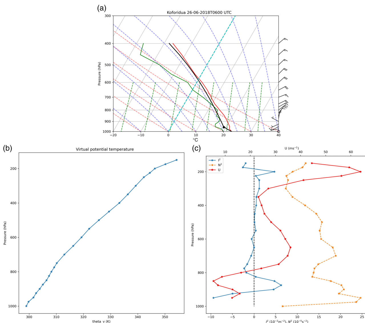
FIGURE 4 (a) SkewT profile at Koforidua, (b) virtual potential temperature and (c) the profile of the Scorer parameter ( I^2 ), Brunt-Vaisala frequency ( N^2 ) and mean wind speed ( U ) at 0600 UTC. ERA5 temperature at atmospheric pressure levels from 1000 hPa to 100 hPa was used to compute the virtual potential temperature, and the inclusion of zonal winds for Scorer parameter and Brunt-Vaisala frequency computations at Koforidua at 26-06-2018T0600 UTC. In addition, the various lines drawn on the SkewT include air temperature (solid red), dewpoint temperature (solid green), parcel profile path (solid black), temperature at lifted condensation level (black dot), zero degree isotherm (dashed turquoise), dry adiabats (dashed red), moist adiabats (dashed blue) and mixing ratio (dashed green). On the right side of the skewT are the wind barbs.
