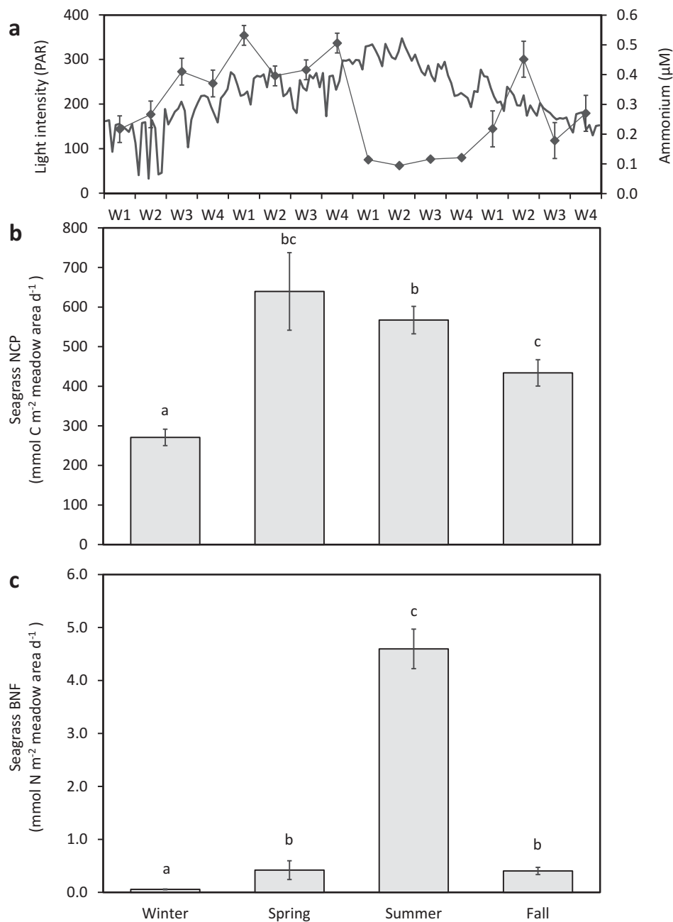
Fig. 3. (a) Daily maximum PAR and NH 4 + concentrations (weekly averages, with 4 weeks in each seasonal period) as representative environmental factors at the study site (10 m water depth); (b) H. stipulacea meadow net community primary production (NCP) and (c) biological N 2 fixation (BNF) in the four seasonal periods. Significant pairwise comparisons for the factor “Season” ( p < 0.05 , PERMANOVA) are indicated as different letters.
