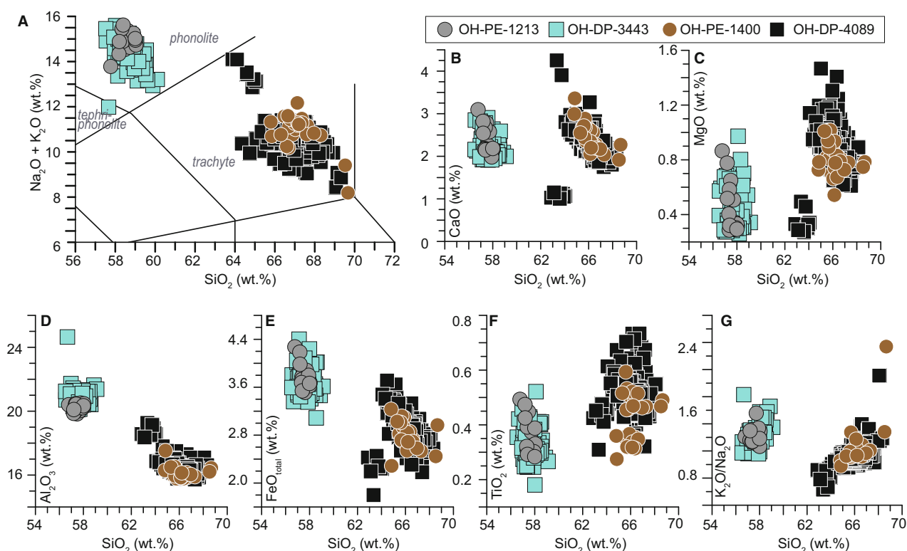
Fig. 4. TAS-diagram according to Le Bas et al. (1986) (A) and bioxide plots (B–G) of glass compositions of tephra layers OH-PE-1213/-1400 and OH-DP-3443/-4089 demonstrating the correlation of respective tephra layers from the Pestani and DEEP sites. Geochemical compositions of OH-DP-3443/-4089 are based on Leicher et al. (2021).
