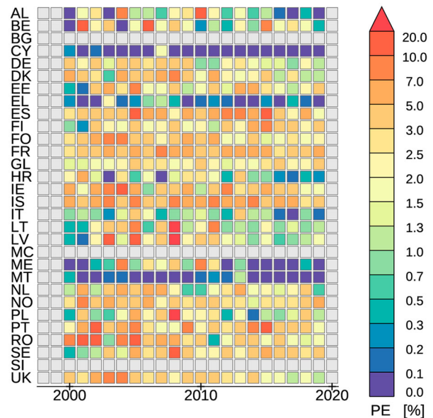
Figure 3.1.5. Time series (2000–2019) of the UNEP (2021) SDG 14.1.1a Level 1 chlorophyll-a deviation sub-indicator based on OC-CCI global chlorophyll-a data (product ref. 3.1.6). Grey boxes identify missing data: reporting was not computed for 1998, 1999 and 2020 (list of countries as for Figure 3.1.4).
