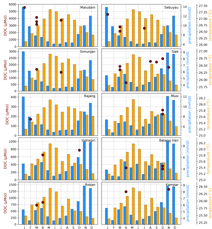
Figure B5. Average DOC concentrations for individual campaigns compared to monthly temperature (Natawa, 2018a; Yasutomi et al., 2011) and precipitation (Natawa, 2018b; Yatagai et al., 2020) data (2005–2015 average) at the location of the respective river. Each panel represents one river.
