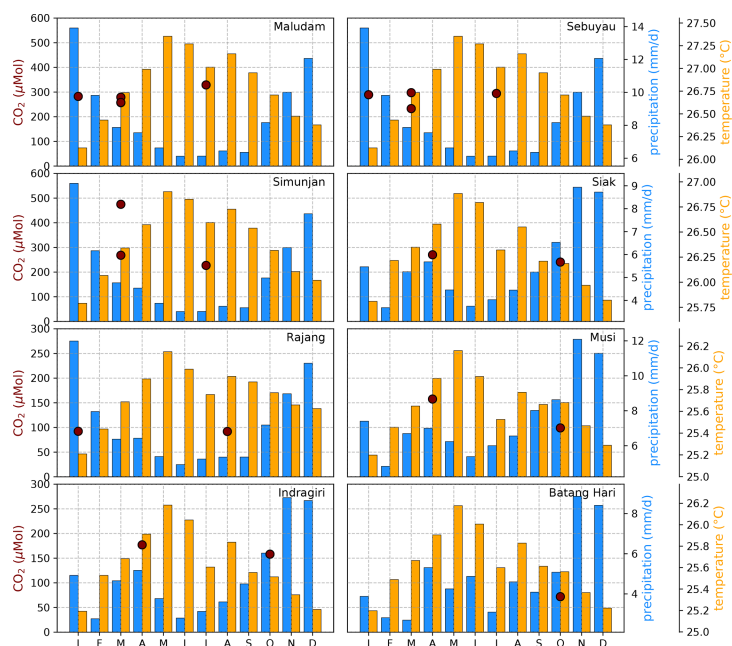
Figure B4. Average CO 2 concentrations for individual campaigns compared to monthly temperature (Natawa, 2018a; Yasutomi et al., 2011) and precipitation (Natawa, 2018b; Yatagai et al., 2020) data (2005–2015 average) at the location of the respective river. Each panel represents one river.
