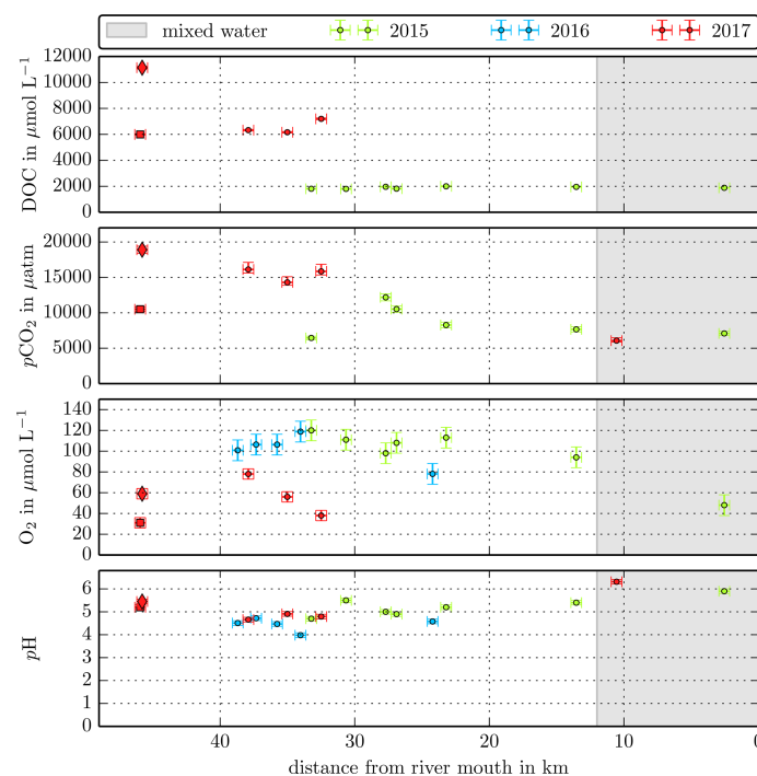
Figure B3. Individual DOC, CO 2 , O 2 , and pH measurements in the Simunjan River versus the distance from the river mouth. Different colours stand for the individual river campaigns, and the grey shaded area indicates regions of S > 1 that were excluded from the data in this study.
