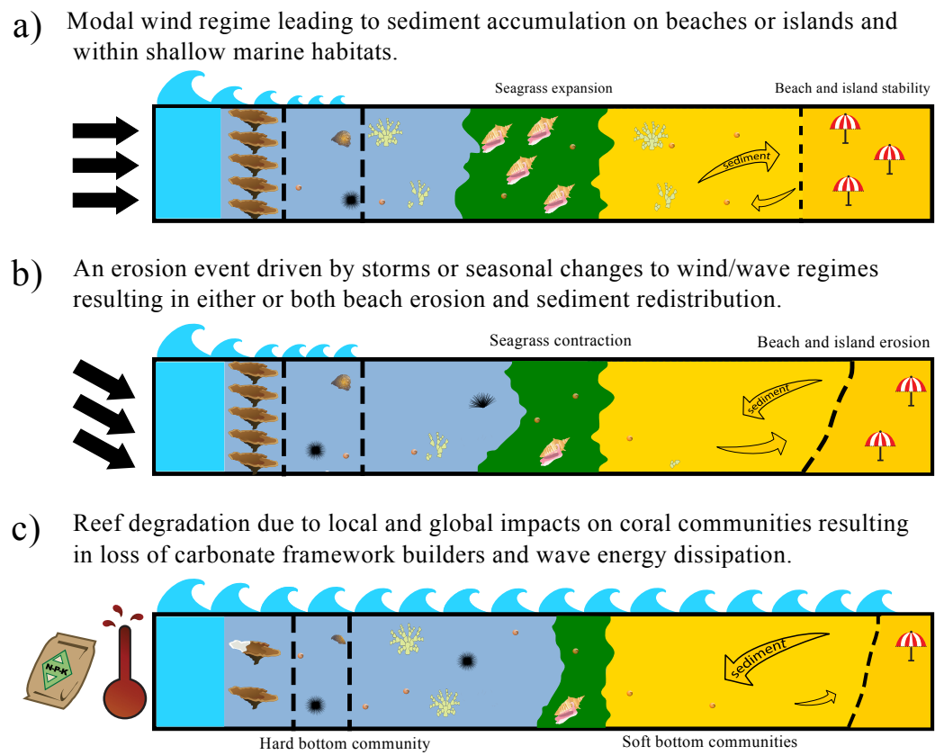
Figure 2 Carbonate framework and sediment production, transport and accumulation altered by variability in the physical system. (A) Fairweather conditions with high coral cover and framework complexity on fore-reef habitats and reef crest dissipate wave energy allowing the development and expansion of lagoonal habitats (e.g., seagrass). These conditions provide a supply of carbonate sediment for beach and island nourishment; (B) episodic or seasonal natural disturbance events may contract lagoonal habitats potentially reducing carbonate sediment production, and redistribute sediment or increase erosion along sedimentary landforms; (C) anthropogenic disturbances due to local (e.g., increased nutrient input) or global (e.g., bleaching) impacts lead to degradation of various reef habitats, especially the reduction of fore-reef and reef crest carbonate framework, which decreases wave energy dissipation, potentially altering sediment production regimes in lagoons and increasing shoreline erosion.
