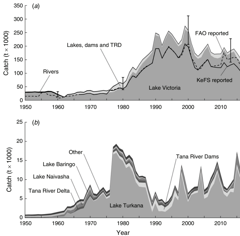
Fig. 2. (a) Total reconstructed freshwater catches for Kenya from 1950 to 2017 by major waterbody category. Catches as reported by the FAO on behalf of Kenya are overlaid as a dashed line, whereas the KeFS nationally reported catches are overlaid as a solid line. Data reliability (uncertainty) bounds are indicated as catch-weighted averages for the 1950–69, 1970–89, 1990–2009 and 2010–17 periods. (b) Total reconstructed freshwater catches for Kenya from 1950 to 2017 for individual waterbodies within the Lakes, Dams and TRD category.
